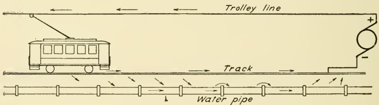
Fig. 210. Diagram Showing Stray Current to Water Pipe
